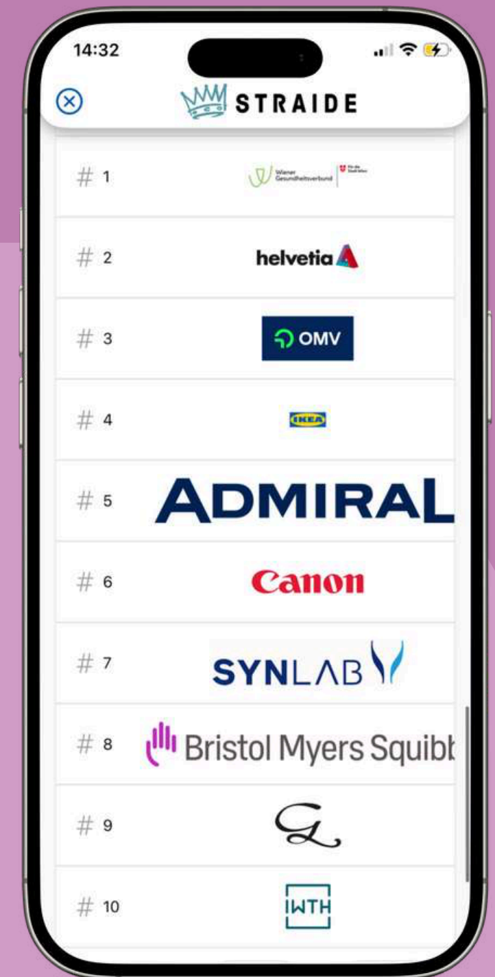
Challenge-Ranking
